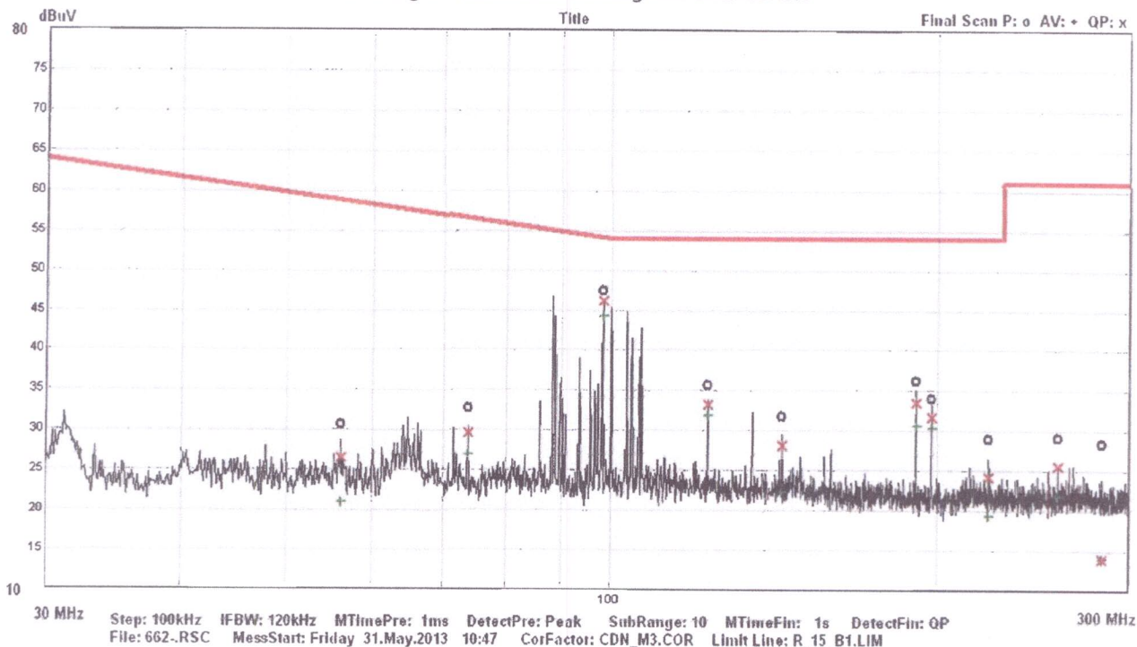
Drawing of Radiated electromagnetic disturbances
